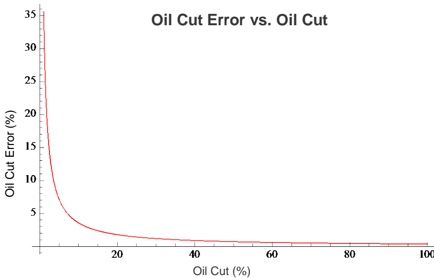
Fig. 2: Plot of the percent error in the oil cut vs. the actual oil cut, based on the \pm 0.001 \text{ g/cm}^3 accuracy of the meter's density measurement. This graph assumes oil density equals 0.823 \text{ g/cm}^3 , water density equals 1.105 \text{ g/cm}^3 and there is no free gas present.
